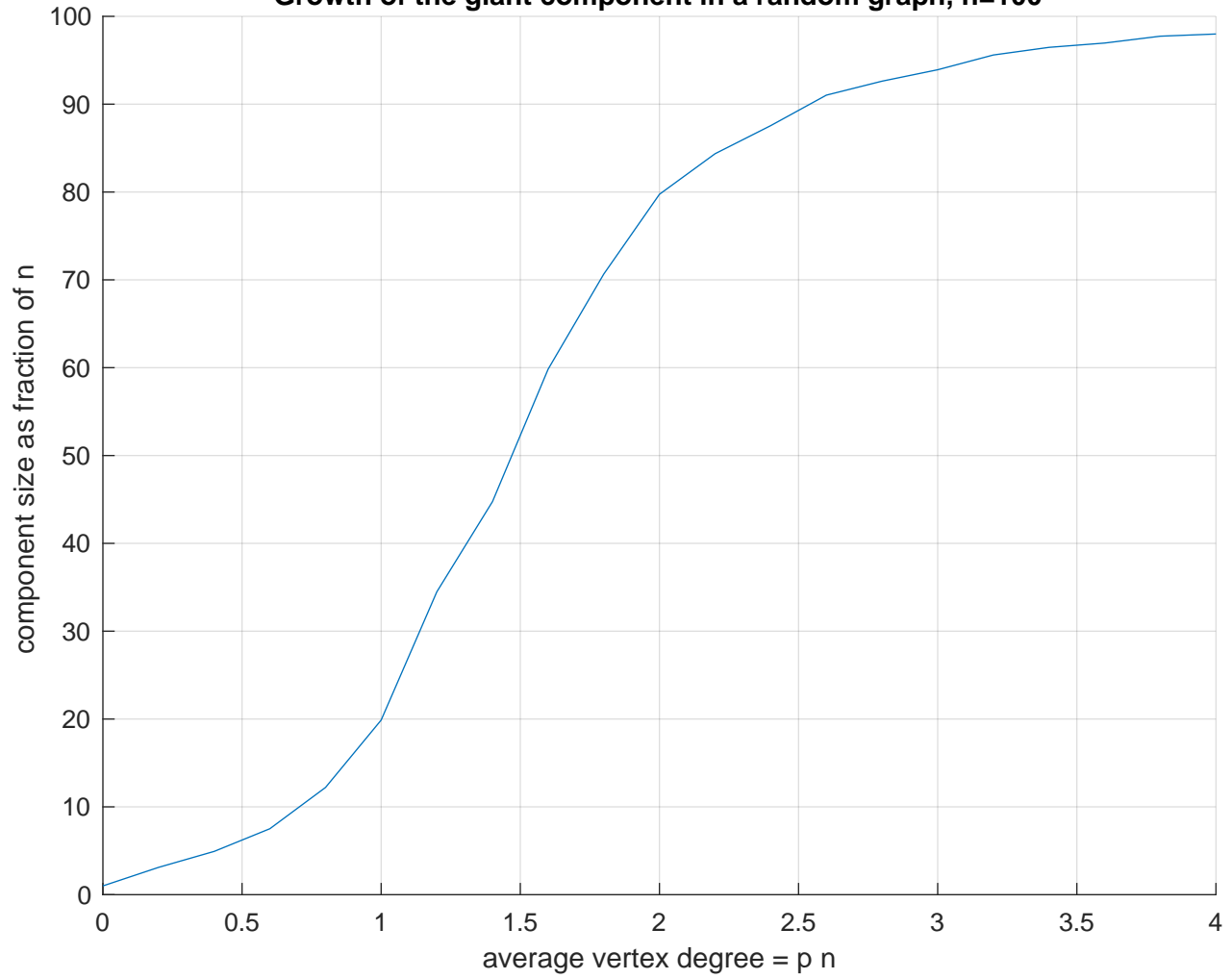
Growth of the giant component in a random graph, n=100
