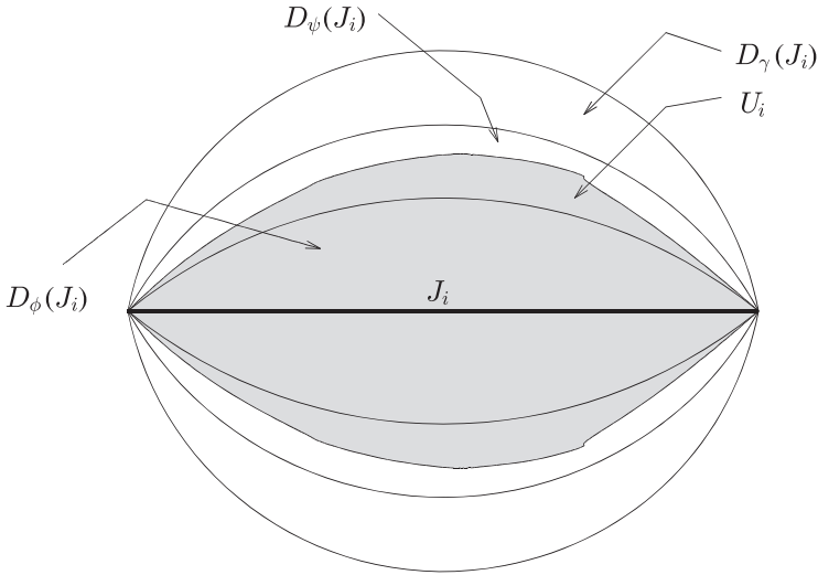
Fig. 3. Geometric domains
