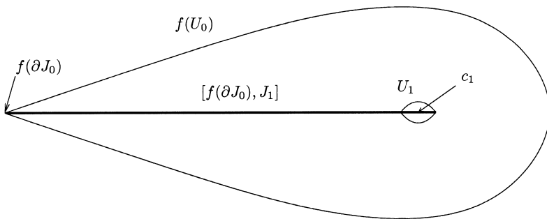
Fig. 4. Domain f(U_0)
