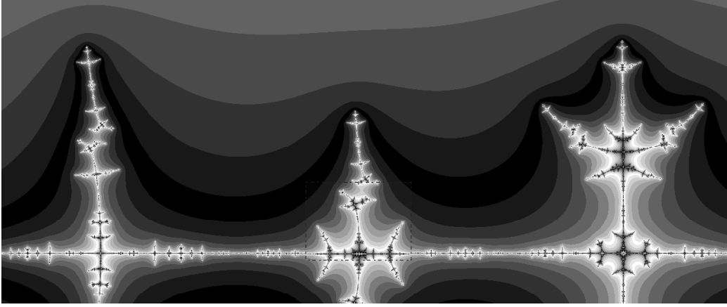
Figure 9. Detail of Figure 8, with different coloring
