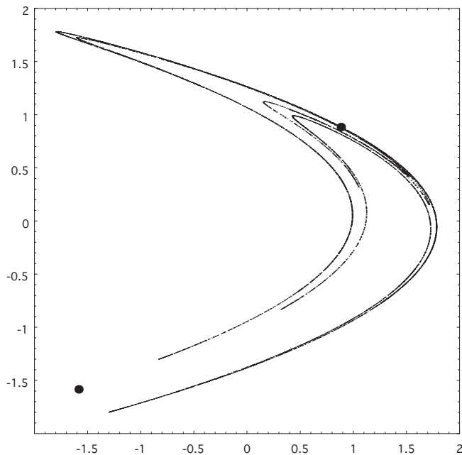
Figure 2. Orbit portrait for h_{a,b} : a = 1.4 , b = -.3
