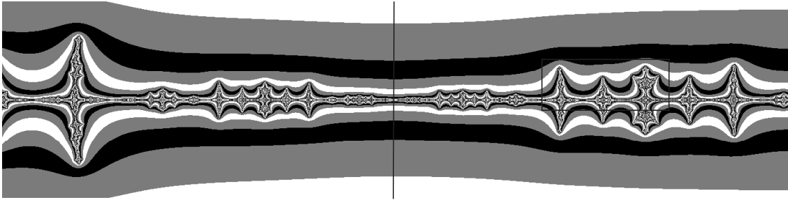
Figure 8. Level sets for G^+ for an unstable slice:* a = 1.4, b = -0.3
