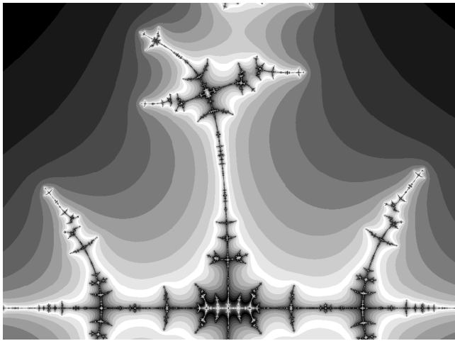
Figure 10. Detail of Figure 9
