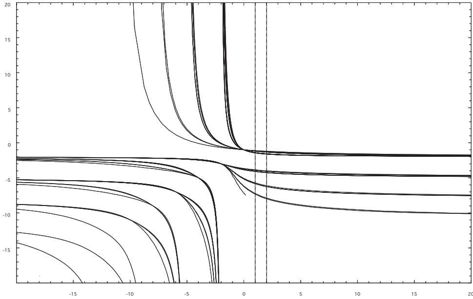
Figure 12. Unstable manifold for f_a : a = -2
