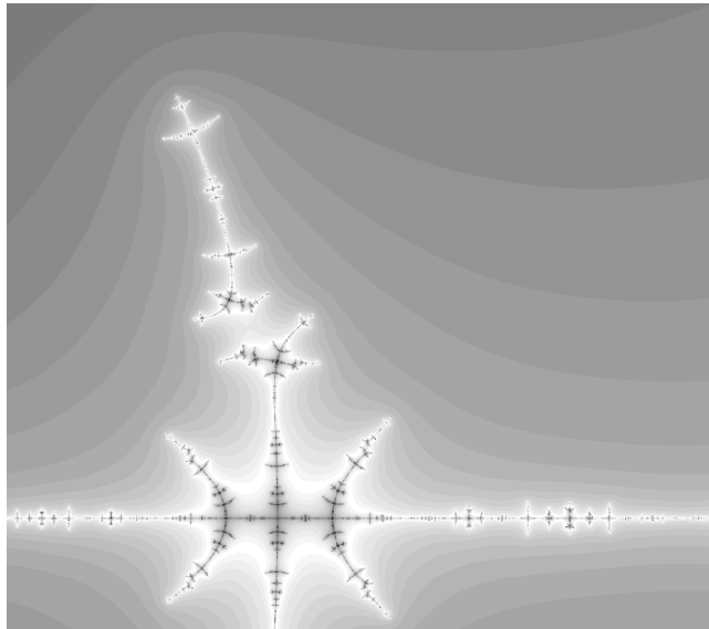
Figure 15. Detail of Figure 14
