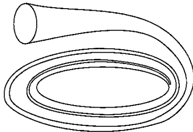
Fig. 7.15. How a non-trivial circle may support no non-trivial covers
