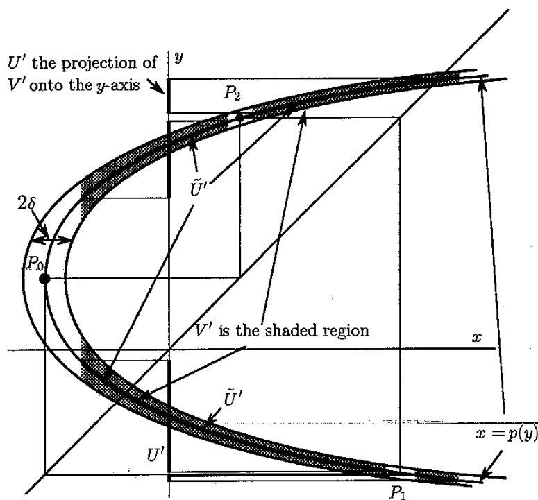
Fig. 4.3. The neighborhood V' of the Julia set \tilde{J}_p \subset C_p
