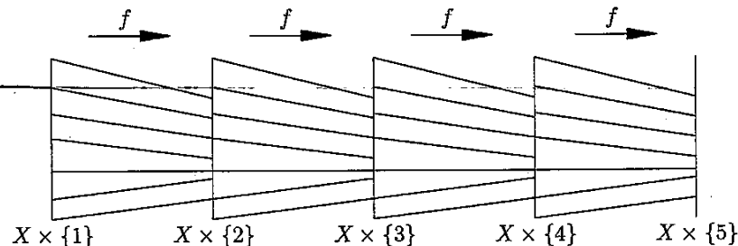
Fig. 1.1. Inductive limit as an increasing union
