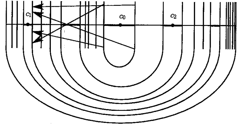
Fig. 8.8. The set ((J_p \cap \mathbb{R}) \times I) \times \{1\} ; the second step in the construction
