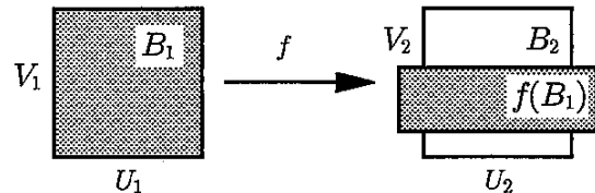
Fig. 3.1. A 1-crossed mapping
