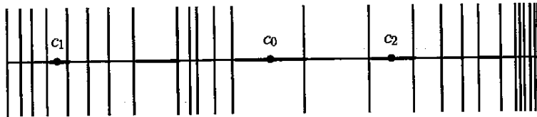
Fig. 8.7. The set (J_p \cap \mathbb{R}) \times I ; the first step in the construction
