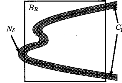
Fig. 4.2. The curve C_p and its neighborhood N_\delta , drawn in \mathbb{R}^2 .
