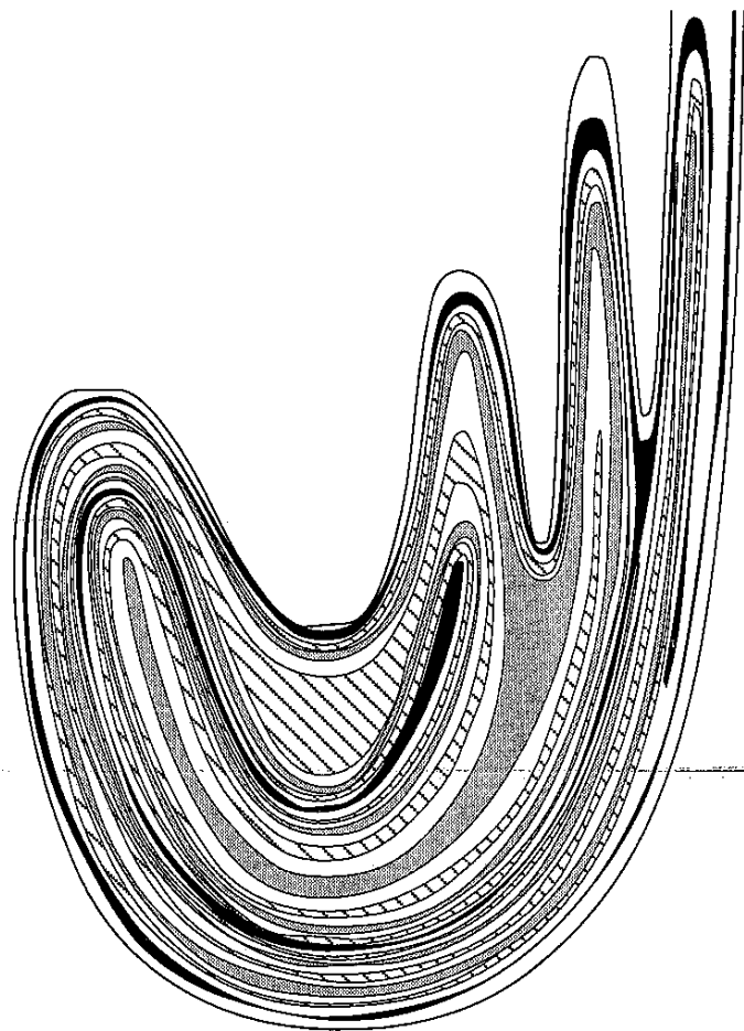
Fig. 8.10. How the basins of the attractive cycle fit to form Lakes of Wada
