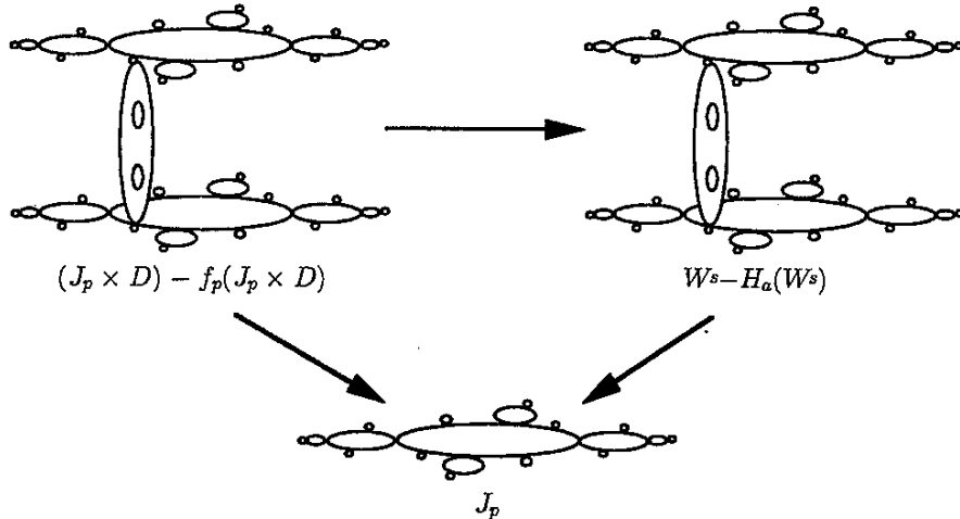
Fig. 6.7. The two fiber bundles. All homeomorphisms which commute with the projection are the identity on the boundary and transform f_p into H .
