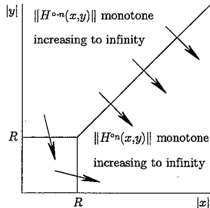
Fig. 4.1. Crude picture of the dynamics of H_a .
