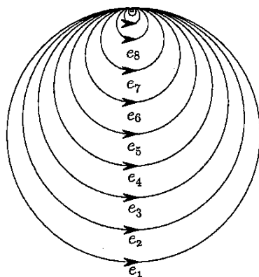
Fig. 7.9. The Hawaiian earring
