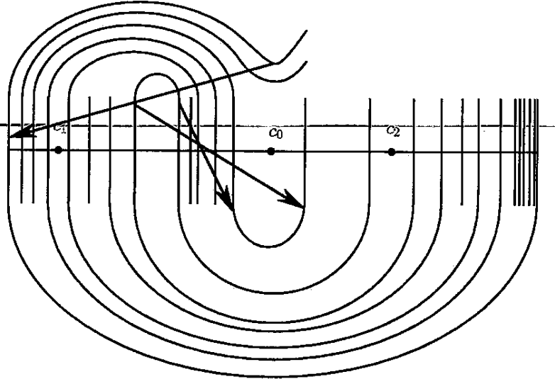
Fig. 8.9. The set ((J_p \cap \mathbb{R}) \times I) \times \{2\} ; the third step in the construction
