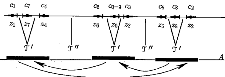
Fig. 8.3. The polynomial z^2 - 1.785866\dots , with an attractive cycle of length 9
