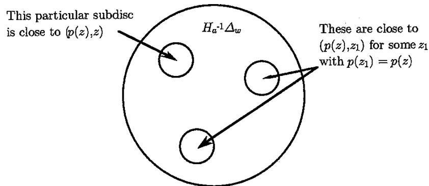
Fig. 4.8. How the image of a vertical disc intersects N_\delta
