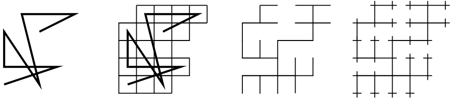
Fig. 4 A continua is covered by dyadic boxes and an approximated tree is formed from the boxes' edges. Some extra segments are added to make every degree 1 or 4 and every edge have length 2^{-D} or 2^{-D-2}
