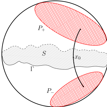
Figure 4.1. The statement of Proposition 4.1. The geodesic segment through x_0 has length \leq w , for w = \arctanh(2\|\Psi\|_{\mathcal{B}}) , and this does not depend on x_0 \in S .
