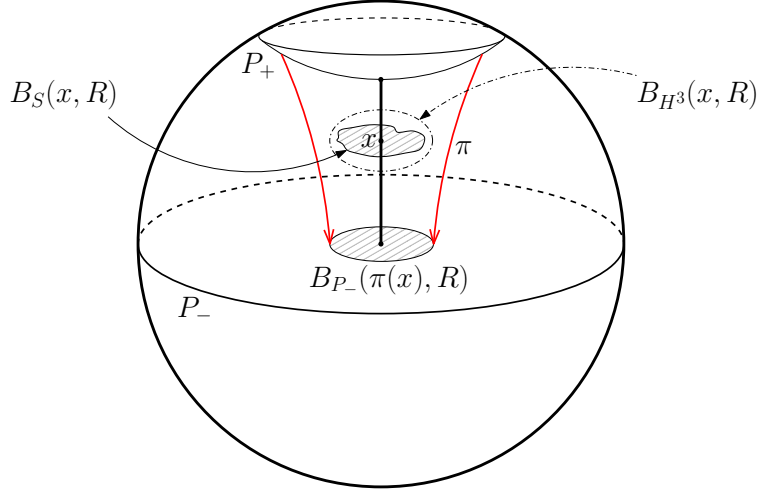
Figure 4.4. Projection to a plane P_- in \mathbb{H}^3 is distance contracting. The dash-dotted ball schematically represents a geodesic ball of \mathbb{H}^3 .
