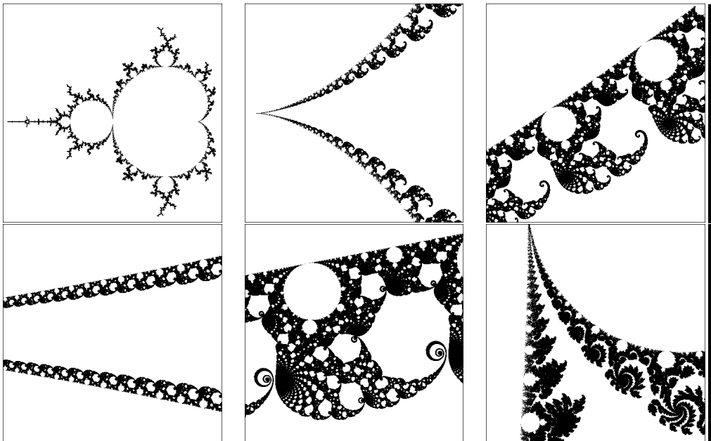
FIGURE 1. The boundary of the Mandelbrot set (top left) and its blow-ups near the cusp c = \frac{1}{4} .
