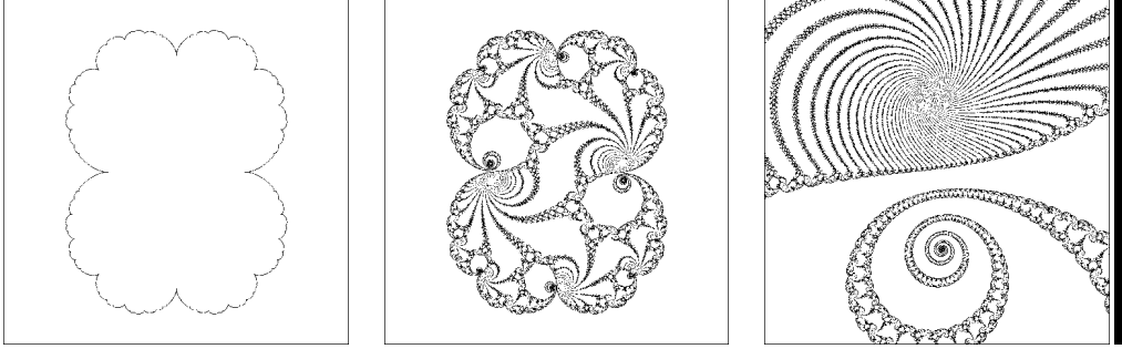
FIGURE 2. The Julia sets for c = \frac{1}{4} (left) and for c = 0.25393 + 0.00048i (middle) and its blow up near the fixed points (right)
