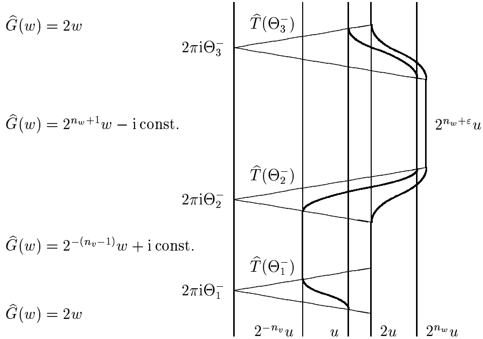
Figure 5.3: Part of the smoothed boundaries and three of the six sectors \hat{T} in the right halfplane, with n_v = k_v - \tilde{k}_v and n_w = n = \tilde{k}_w - k_w . The image assumes \tilde{k}_w > 2k_w , otherwise the boundaries will have additional bumps between \Theta_1^- and \Theta_2^- .
