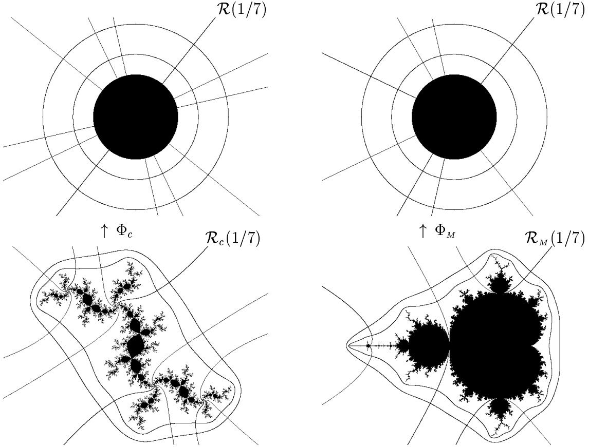
Figure 1: A connected filled-in Julia set \mathcal{K}_c and the Mandelbrot set \mathcal{M} . External rays and equipotential lines are defined as preimages of straight rays and circles under the conformal mappings \Phi_c : \hat{\mathbb{C}} \setminus \mathcal{K}_c \rightarrow \hat{\mathbb{C}} \setminus \overline{\mathbb{D}} and \Phi_M : \hat{\mathbb{C}} \setminus \mathcal{M} \rightarrow \hat{\mathbb{C}} \setminus \overline{\mathbb{D}} , respectively.
