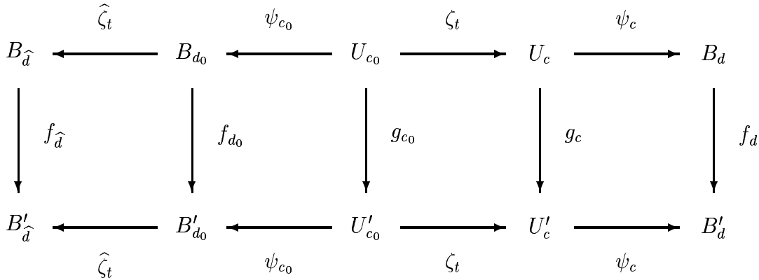
Figure 5.6: This commuting diagram proves that the homeomorphism h is analytic in a non-hyperbolic component \Omega . We have d_0 = h(c_0) , d = h(c) , c = \gamma(t) and \widehat{d} = \widehat{\gamma}(t) .
