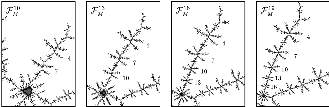
Figure 8.6: Parts of rescaled parameter frames \rho_a^n(\mathcal{F}_M^n - a) . The numbers m mark the subframes \rho_a^n(\mathcal{F}_M^{n,m} - a) according to (8.11). Now we have \rho_a^{n+3}(\mathcal{F}_M^{n+3,4} - a) \approx \rho_a^n(\mathcal{F}_M^{n,4} - a) and \rho_a^{n+3}(\mathcal{F}_M^{n+3,7} - a) \approx \rho_a^n(\mathcal{F}_M^{n,7} - a) , but h : \mathcal{F}_M^{n+3,7} \rightarrow \mathcal{F}_M^{n,4} shows that h is not asymptotically linear at a . Observe that the arms of \mathcal{F}_M^{19} already look like those of \mathcal{K}_a in Figure 8.4. The rescaled centers are converging to \rho_a^4 \frac{\phi_a(0)}{w'(a)} , and the vertices of the frames are of the form c_n \pm K \rho_a^{-3n/2} , thus they are converging to the same point under the rescaling by \rho_a^n . They have different limits under rescaling by \rho_a^{3n/2} , cf. Section 8.6.
