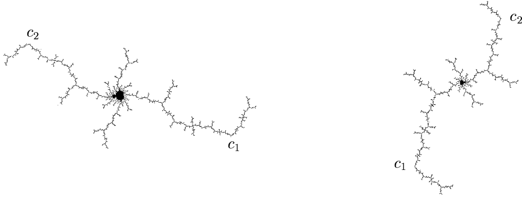
Figure 7.3: The largest frames on the edges of orders 5 and 6 that are attached to the edge of order 4 at its upper vertex (cf. Figure 8.3). Observe that there are two additional arms of length comparable to the arms at the vertices, which are missing in the frames on the edge of order 4, cf. Figure 7.5. Note that in the present figure the parts of \mathcal{M} before c_1 and behind c_2 are cut away, while the corresponding parts are shown in Figure 7.5.
