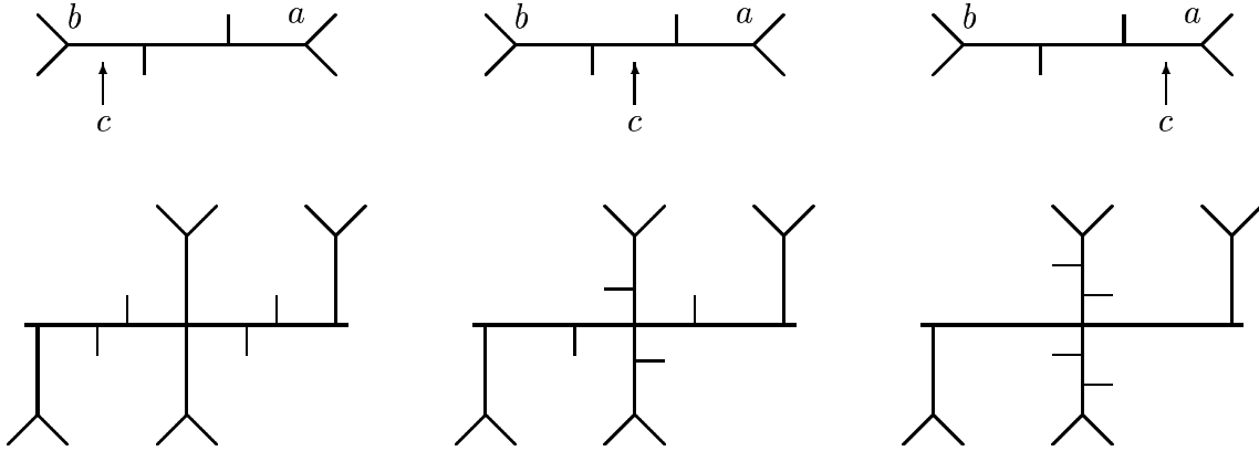
Figure 7.4: Bifurcations of subframes in \mathcal{F}_1^c(1, 0) or in any dynamic frame, as the parameter c varies in the edge \mathcal{E}_M of order 4. In the first and third case, there are corresponding parameter subframes.
