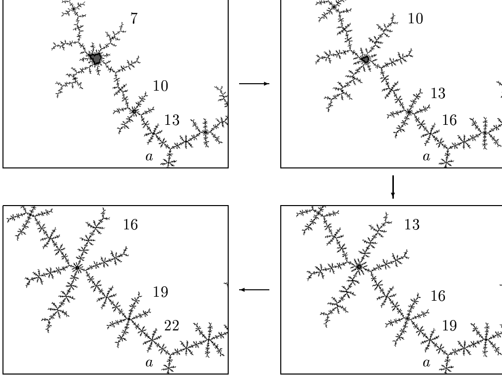
Figure 8.5: In the four images a neighborhood of a = \gamma_M(9/56) is blown up successively by a factor \rho_a^3 with \rho_a = f'_a(\alpha_a) = 2\alpha_a . The parts of \rho_a^n(\mathcal{M} - a) in some fixed rectangle are shown for values of n increasing by 3, i.e. the disk from Lemma 8.4 is replaced with the rectangle. Under this rescaling each branch of \mathcal{M} converges to a branch of Y_a . The argument of \rho_a^3 is very small, but in fact the three branches behave like logarithmic spirals at a , turning around a an infinite number of times at exponentially small distances. The numbers are the orders of the maximal frames \mathcal{F}_M^n according to (8.10).
