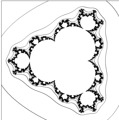
Figure 2. The “Multibrot set” for degree n = 4 , that is the connectedness locus in the b -parameter plane for the family of unicritical polynomial maps z \mapsto z^4 + b . (See for example [LS2].) Note the (n - 1) -fold rotational symmetry. The corresponding figure in the b^3 -plane is shown in Figure 1a.
