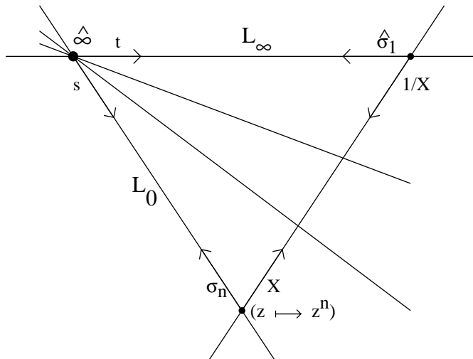
Figure 11. Schematic picture of the compactified moduli space \widehat{\mathcal{M}} \cup \widehat{\infty} , with a singular point at \widehat{\infty} , showing the three overlapping systems of coordinates.
