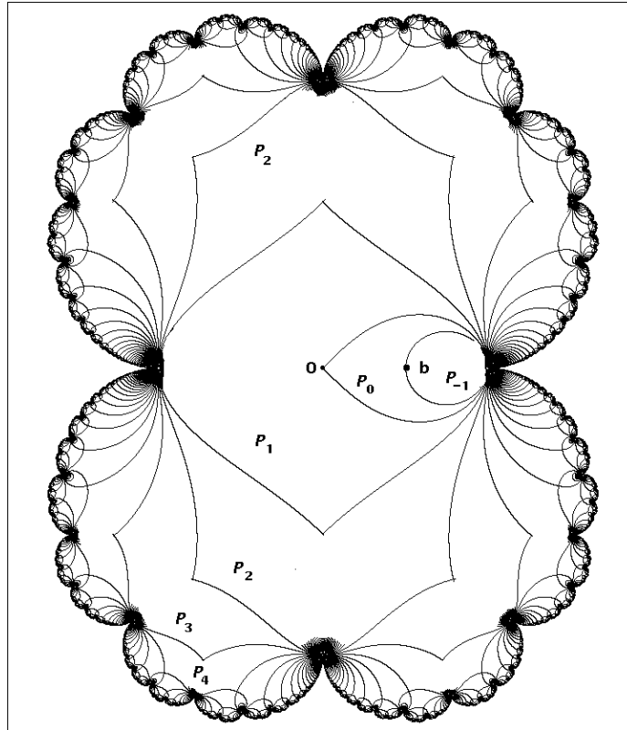
Figure 5. The regions \mathcal{P}_0 \subset \mathcal{P}_1 \subset \dots for the quadratic case n = 2 . (Note: In the region outside of \mathcal{P}_4 , all of the iterated preimages of \partial\mathcal{P}_0 have been drawn in, so that this figure looks more complicated near the basin boundary.)
