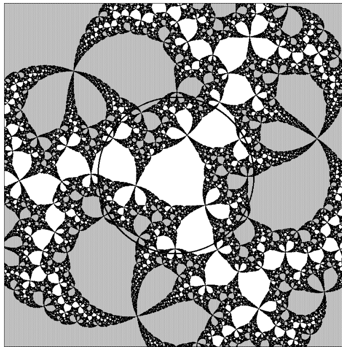
Figure 8. Dynamic plane for a degree n = 3 bicritical map which commutes with the antipodal map, with the unit circle drawn in. (Parameters X = -.235 , Y = .213 .) There are two attracting period 4 orbits. The antipodal map of \hat{\mathbb{C}} , reflection in the unit circle composed with the 180^\circ rotation, interchanges the two attracting basins, which are colored white and grey respectively. The Julia set, like that for an arbitrary degree n bicritical map, has n -fold rotational symmetry. It is conjectured that this particular map can be obtained as a mating of the form (z^3 + b) \perp\!\!\!\perp (z^3 - \bar{b}) , with b \approx .584 - .270i . (Compare [T].)
