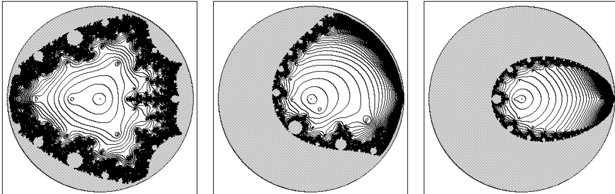
Figure 10. Pictures in the disk |\lambda| < 1 for X equal to -.2 , .2i and .2 respectively, for degree n = 2 . (Compare 6.3.) The connectedness locus is shaded grey; while the curves in the shift locus indicate the number of iterations needed for both critical orbits to reach a small neighborhood of the attracting fixed point.
