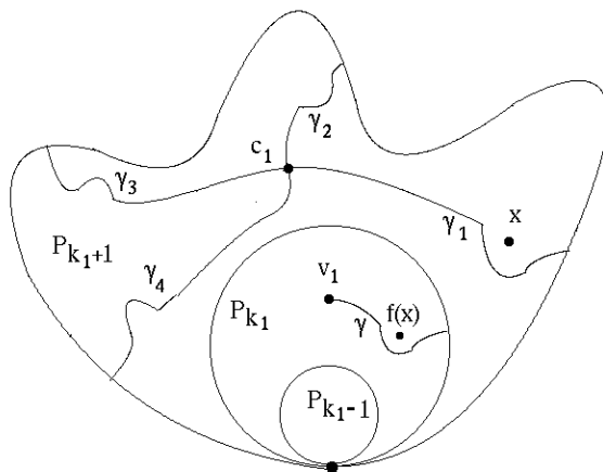
Figure 4. This shows the three petals P_{k_1-1} , P_{k_1} , and P_{k_1+1} . The point x = f^{\circ(k_2-k_1)}(c_2) belongs to the orbit of the second critical point. A path \gamma from v_1 to \partial P_{k_1} within P_{k_1} \setminus (\overline{P_{k_1-1}} \cup \{f(x)\}) lifts to n distinct paths \gamma_i from c_1 to \partial P_{k_1+1} . We must choose this path \gamma so that x and P_{k_1} belong to the same connected component of P_{k_1+1} \setminus (\gamma_1 \cup \dots \cup \gamma_n) .
