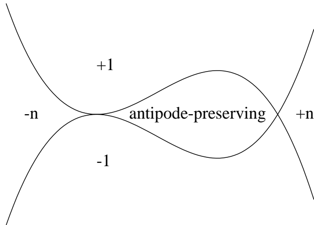
Figure 7. Symmetry locus in the real (X, Y) -plane for degree n = 3 , with the five complementary domains appropriately labeled.
