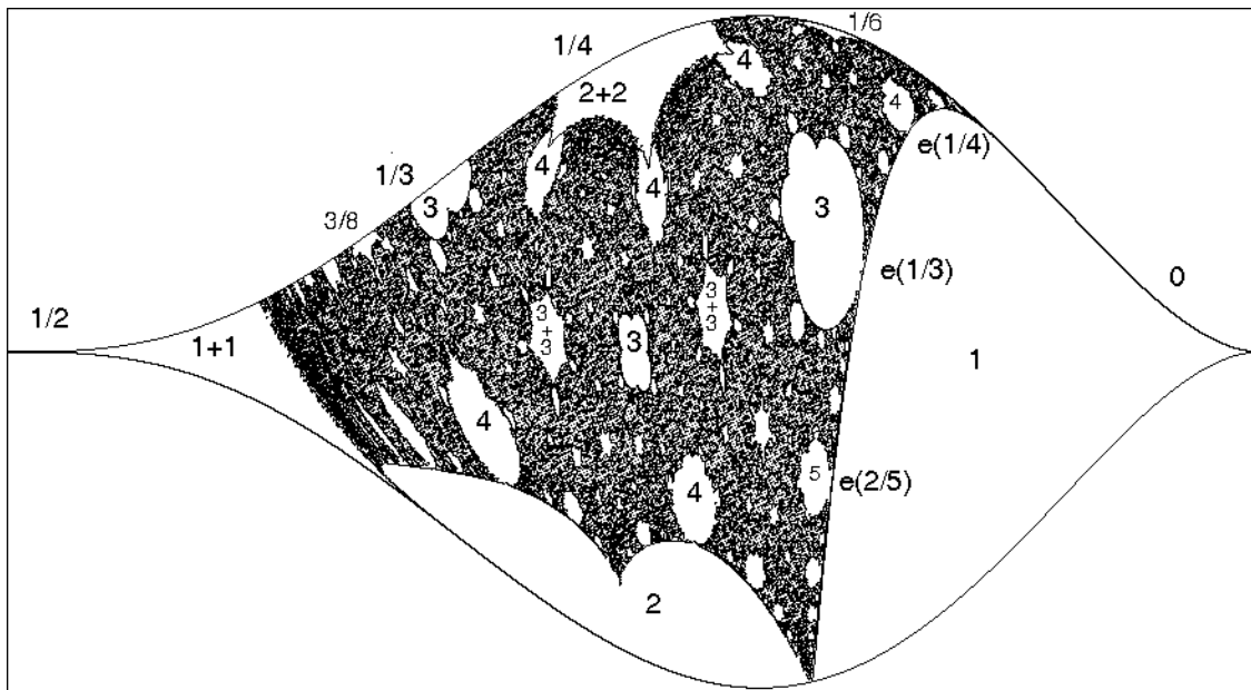
Figure 9. Antipode-preserving region of the (X, Y) -plane for degrees 3 and 5, with periods of the larger hyperbolic components labeled. (Note that the components of type p + p have a tricorn-like geometry. Compare [NS]) Along the top edge, these maps give rise to degree one circle homeomorphisms, with rotation number as indicated. Also, along the edge of the principal hyperbolic component, the multiplier of one of the two indifferent fixed points is indicated, using the notation e(x) = e^{2\pi i x} .
