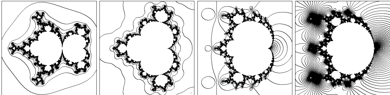
Figure 1. Pictures of \mathcal{C} \cap \text{Per}_1(\lambda) for \lambda = 0, .01, 0.5 , and \lambda = 1 respectively, for the degree n = 4 . The configuration deforms continuously for 0 < \lambda < 1 , and conjecturally as \lambda \rightarrow 1 also. However, there is a qualitative difference between the first and second pictures due to the fact that as \lambda \rightarrow 0 the curve \text{Per}_1(\lambda) converges not towards \text{Per}_1(0) but rather towards an (n - 1) -fold branched covering of \text{Per}_1(0) as shown in Figure 2. Thus Figure 1b is a somewhat squashed version of Figure 2. The surrounding curves in the 5a, 5b, 5c represent equal rates of convergence towards the attracting fixed point for the more slowly converging critical point. (For the corresponding curves in Figure 1d, see 4.3 below.)
