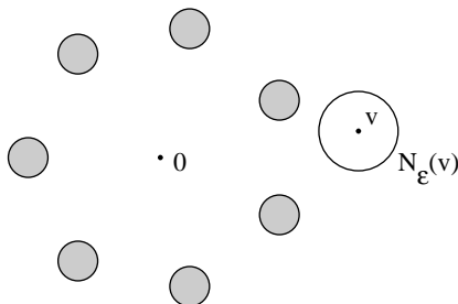
Figure 12. Dynamics for (f) near \widehat{\infty} . Here the critical points are at 0 and \infty , while the critical values as well as the attracting fixed point are in the disk N_\epsilon(v) . The Julia set is contained in the n shaded disks \overline{U}_i , each of which maps diffeomorphically onto the complement \widehat{\mathbb{C}} \setminus \overline{N}_\epsilon(v) . As (f) \rightarrow \widehat{\infty} , each of these n + 1 disks shrinks to a point.
