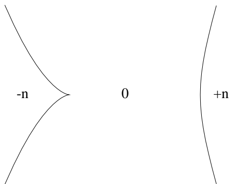
Figure 6. Symmetry locus in the real (X, Y) -plane for degree n = 2 . The three complementary domains are labeled according to the degree of the associated map from the circle of real points to itself. The picture for higher even values of n would have another cusp, corresponding to (z \mapsto z^n) , but would otherwise be similar.
