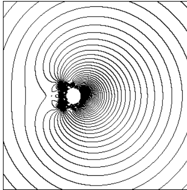
Figure 3. Another picture of \mathcal{C} \cap \text{Per}_1(1) in the degree 4 case, showing a much larger region in order to illustrate behavior near infinity.
