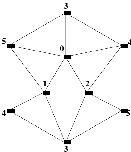
FIGURE 1. The Minimal Triangulation of \mathbb{R}\mathbb{P}^2
