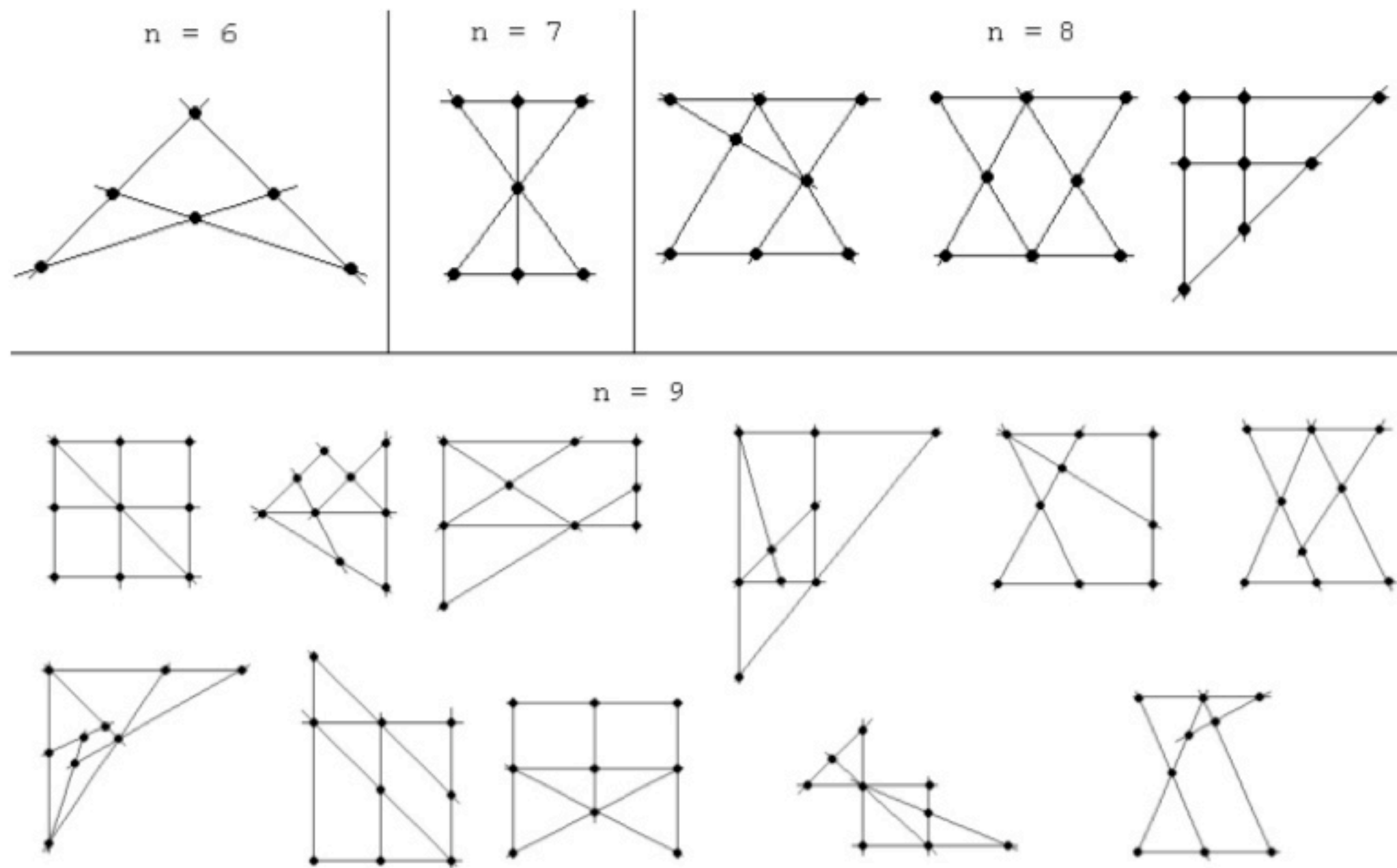
FIGURE 1. All strong hypergraphs for small n were found by Scheidwasser [Sch] using computer search. There are 93 hypergraphs for n = 10 , 1027 hypergraphs for n = 11 , and so on.
