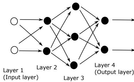
Fig. 2.3 A network with four layers.
