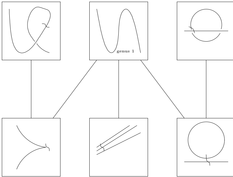
FIGURE 1. Irreducible components and other interesting loci in \overline{\mathcal{M}}_1(\mathbb{P}^2, 3) ; the little squiggle in each panel represents a contracted genus-curve
