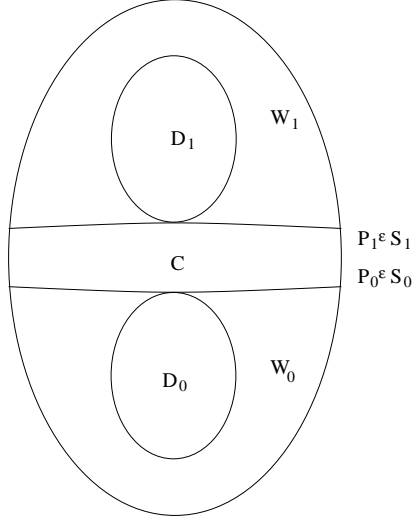
FIG. 5: Partition de \mathbb{P}(\mathbb{C}_p) .
