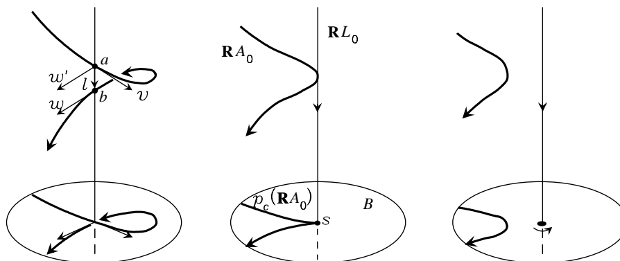
FIGURE 4. Real algebraic version of the first Reidemeister move.
