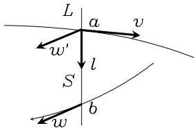
FIGURE 2. Construction of the frame v, l, w' .
