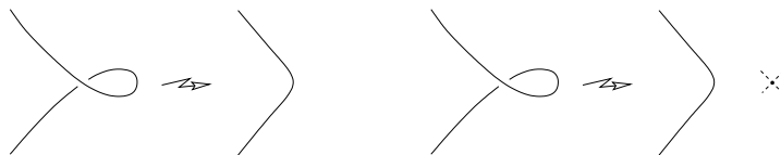
FIGURE 1. Topological (left) and real algebraic (right) versions of the first Reidemeister move. At the solitary crossing point, which is on the right hand side of the picture, the conjugate imaginary branches are indicated by dashed segments, according to an out-dated tradition of Analytic Geometry.
